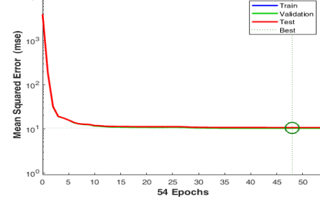
Figure 3: Neural network performance
